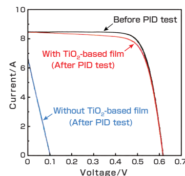
The I-V curves for a standard Si photovoltaic module and a PID-resistant module before and after the PID test by applying -1000 V at 85 °C for 2 h
