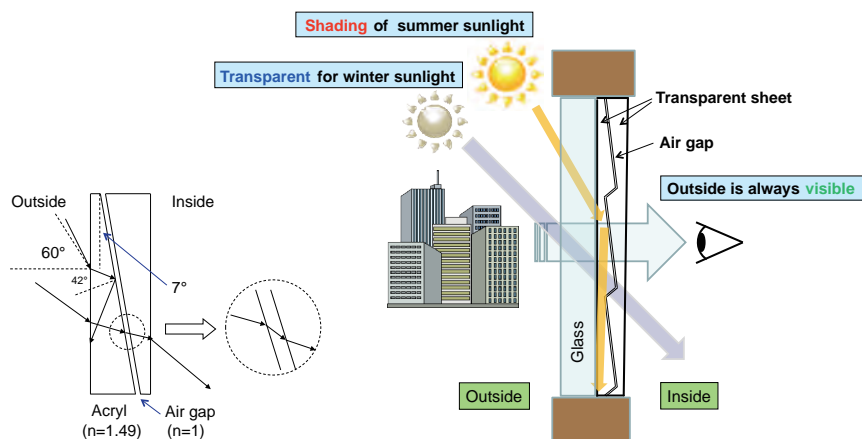
Basic structure of the total-reflection light-control sheet (left) and structure and function of the automatic light-control sheet (right)
