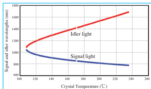
Fig 1: Temperature tuning curve of the continuous-wave optical parametric oscillator
