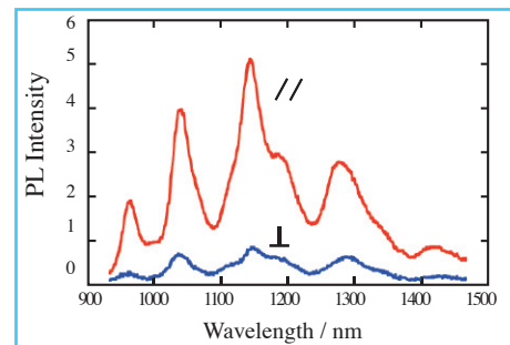
Fig 2: Thin film of isolated and aligned SWNTs generates photoluminescence (PL) strongly polarized in the alignment direction. Each PL peak corresponds to a bandgap optical transition in semiconducting SWNTs. If bundled, tubes would not emit light because of excitation quenching induced by inter-tube interactions.
