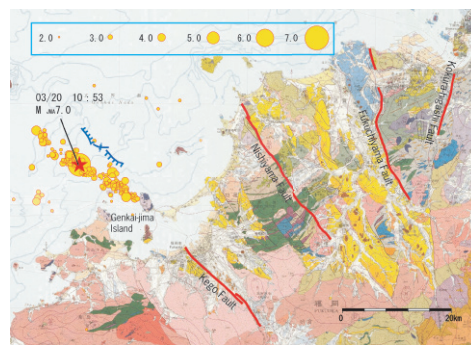
Fig 1: Geological map of Northern Kyusyu and Epicentral distribution of aftershocks occurred in Genkai-Nada in March 20th, 2005(10:53:40-17:58:39). (Epicentral data provided from National Research Institute for Earth Science and Disaster Prevention).
