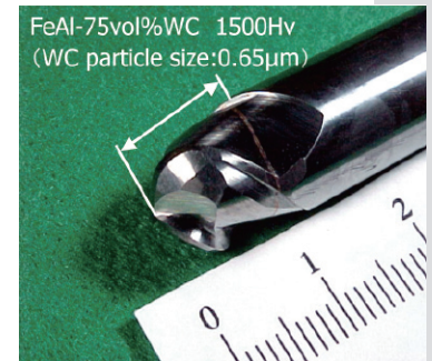
Fig 2: An apparatus of FeAl-75vol% end-mill.
