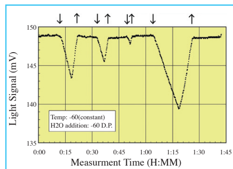
Fig 2: Response of the optical intensity against the moist sample gas. Switching to the sample from dry gas is indicated by down-arrows.
