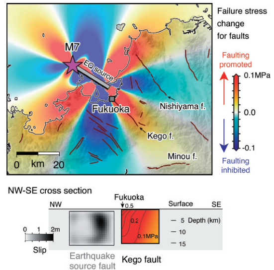
Figure: Failure stress change resolved on faults in the crust (upper panel) and onto the Kego fault beneath the city of Fukuoka (lower panel) caused by the Fukuoka-ken-seiho-oki earthquake.
