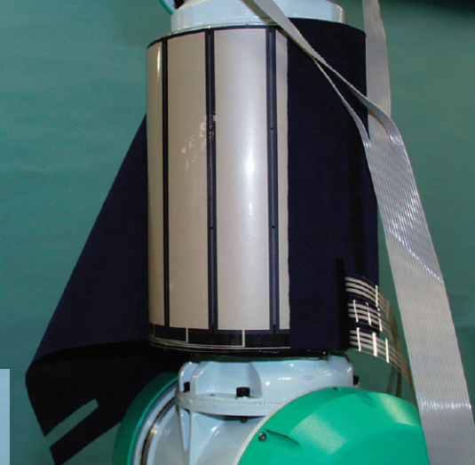
Photo 1: Sensor sheet and the fourth link cuticle Characteristics of the sensor sheet attached are:
