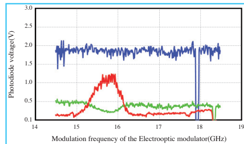
Fig 2: Observed Doppler-broadened signal from the Cs-D 2 line (852nm) The transition from a ground state hyperfine level F=4 to excited states F'=3,4,5 was observed. An electrooptic modulator was used for continuous frequency tuning. Blue line: signal light intensity, Green line: light intensity transmitted through the cell, Red line: fluorescence intensity from the cell. The light was blocked at 17.9 GHz and 18.3 GHz for the zero-level calibration of photodetectors.
